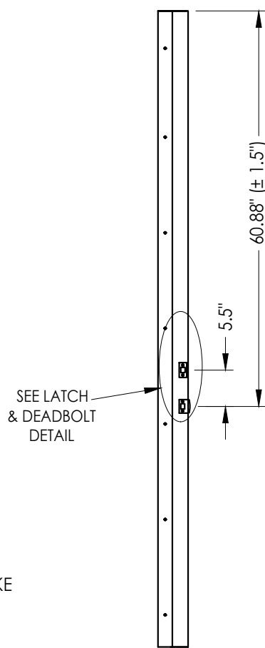
STRIKE JAMB Latch and Deadbolt 5-1/2" ON CENTER
