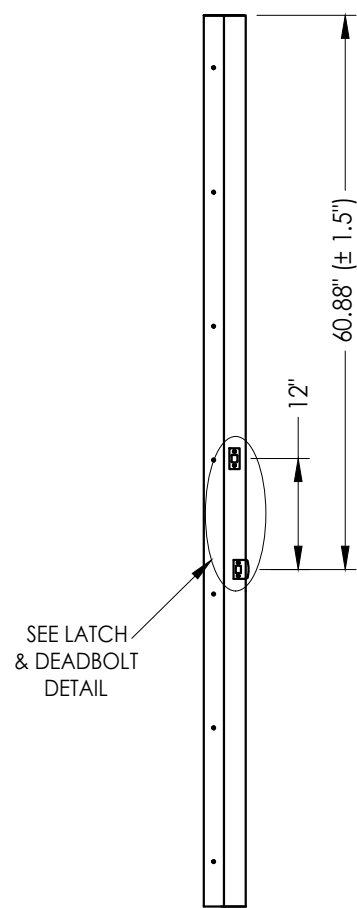
STRIKE JAMB Latch and Deadbolt 12" ON CENTER
