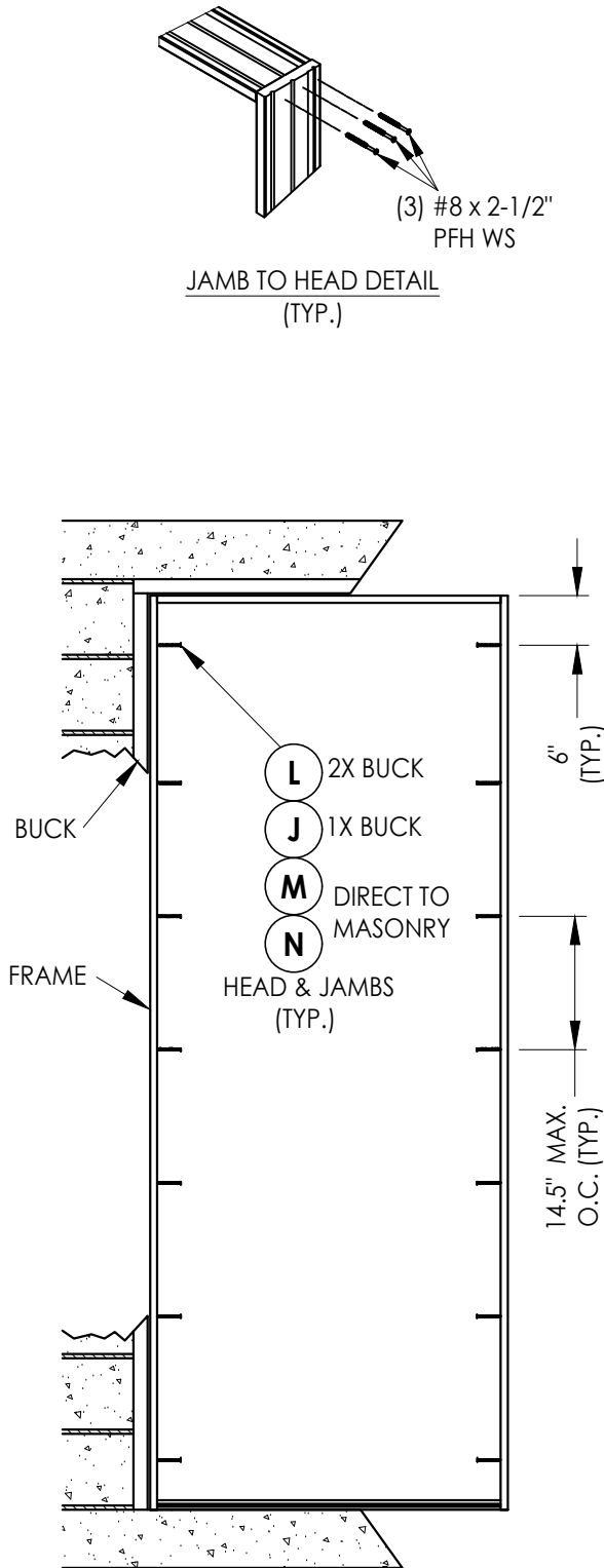
FRAME ANCHORING
